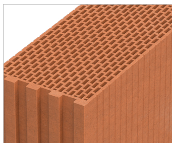
Vertically perforated brick
